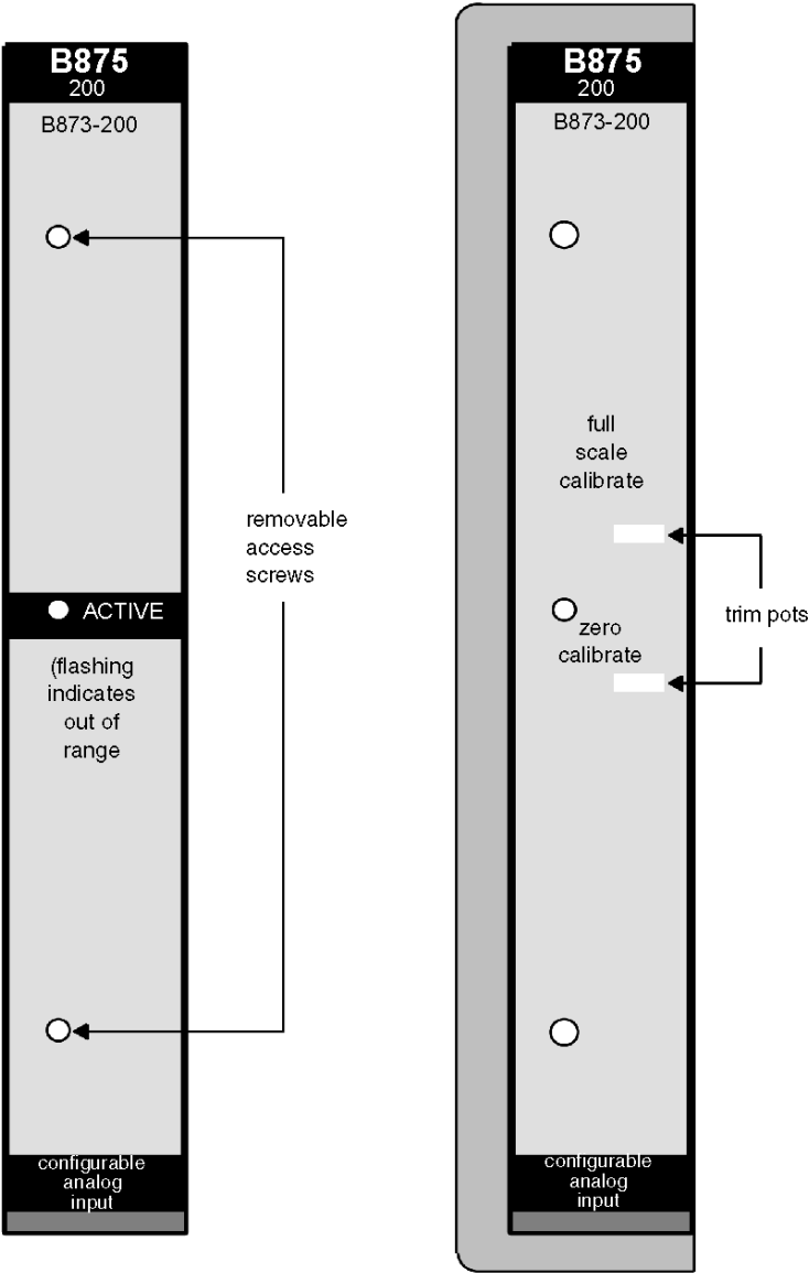
Location of trim pot, diagram
