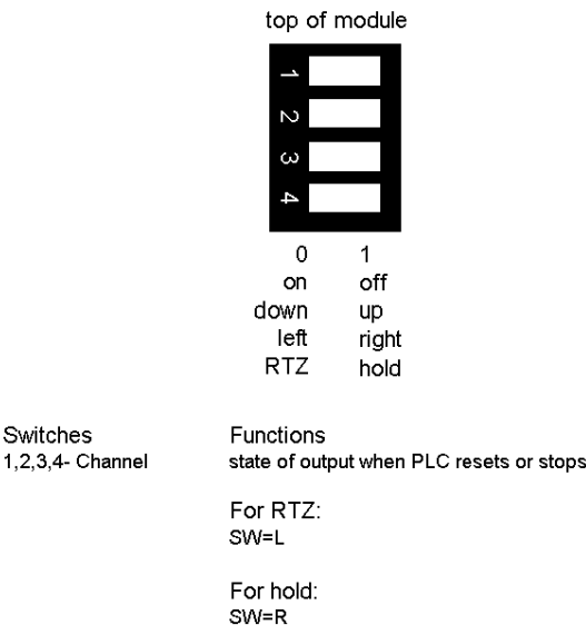
4- Position DIP- Switches
