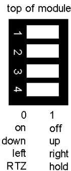
4- Position DIP- Switches
