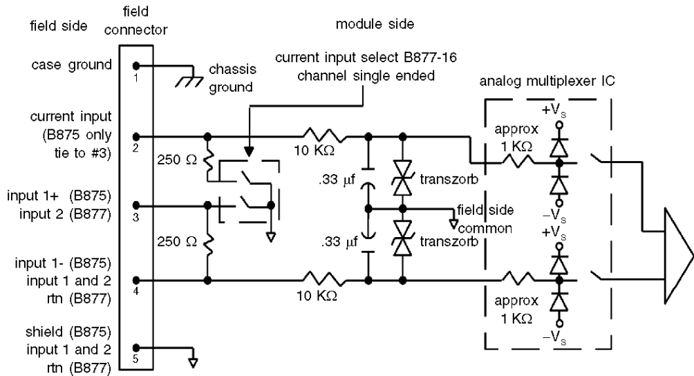
B875-111 Analog input module, simplified schematic diagram
