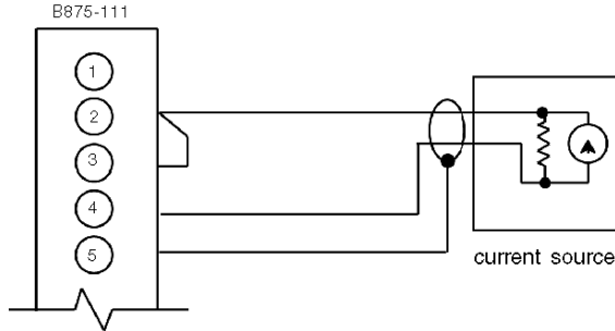
Field connector jumper diagram
