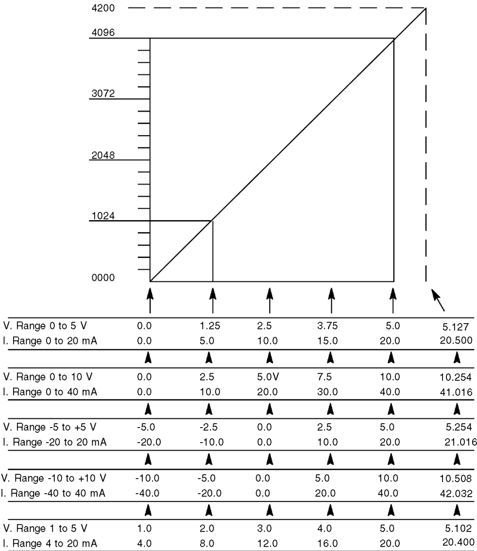
B875-102 Input Signal vs. Output Data (Raw Binary Format)
